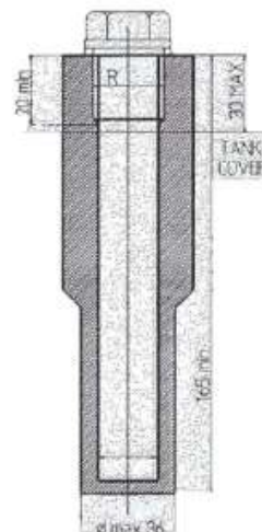
Figure 4 Dimensions of thermometer pockets
