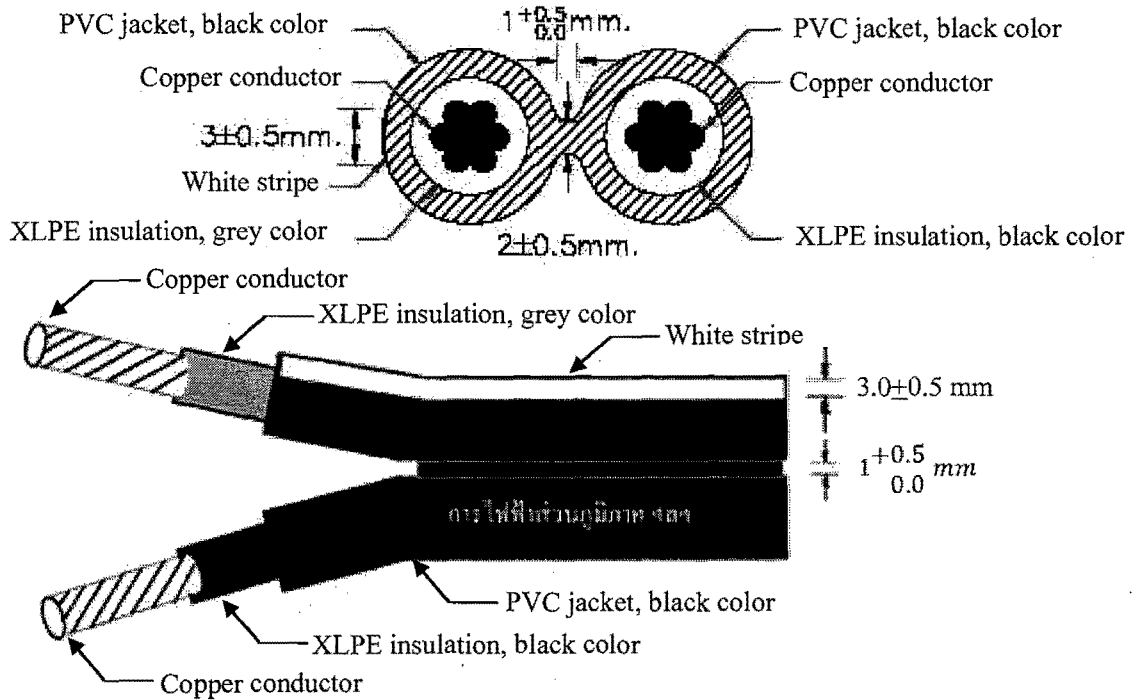
Figure 1 Construction and marking of XLPE insulated and PVC jacketed cable
