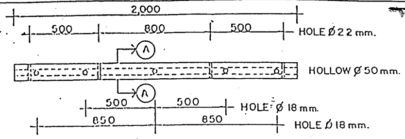
1 : 25 SECTION (A)-(A) 1 : 5 PRESTRESSED CROSSARM 120x120x2,000 mm
