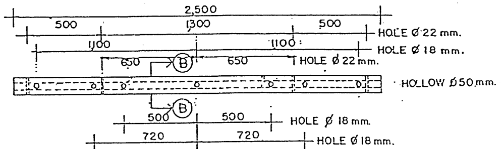
1 : 25 SECTION (B)-(B) 1 : 5 PRESTRESSED CROSSARM 120x120x2,500 mm
