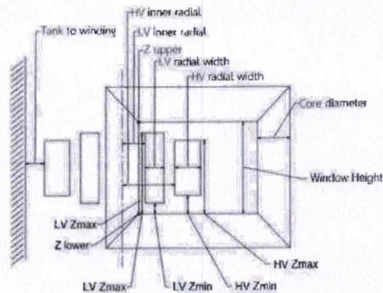
Figure 7: Core and coil constructions.
