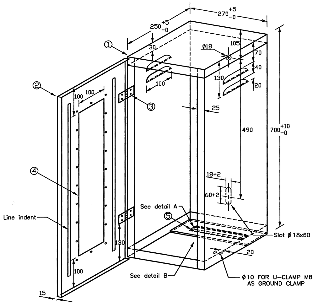
Meter cabinet, for two (2) single-phase electronic energy meters, outdoor installation
