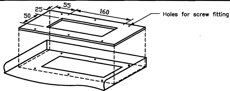
Detail B : Detail of Electrical knockout
