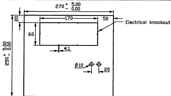
Detail B : Detail of Electrical knockout
