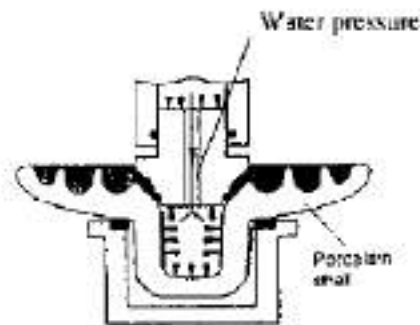
Hydraulic inner pressure test
