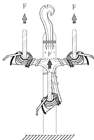
Figure 2 Pulling test arrangement
