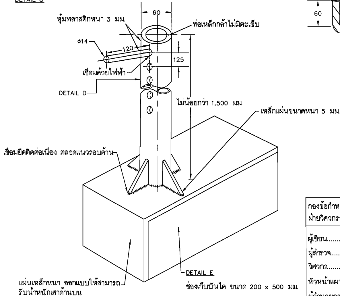
DETAIL C
